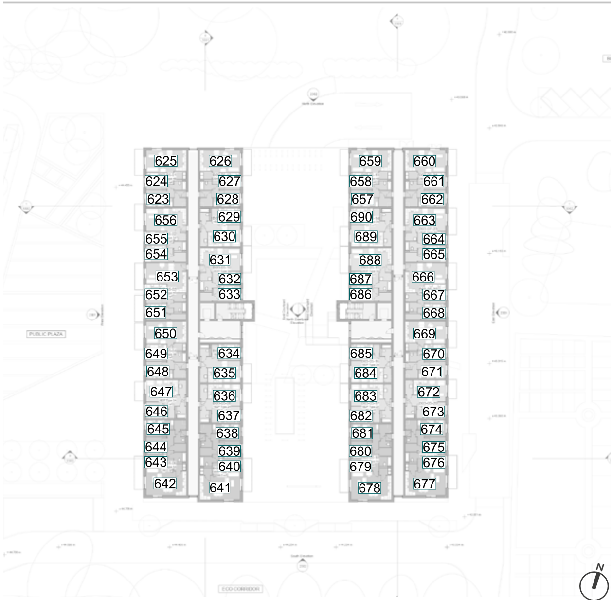
Fig. 27: Floor Plan
