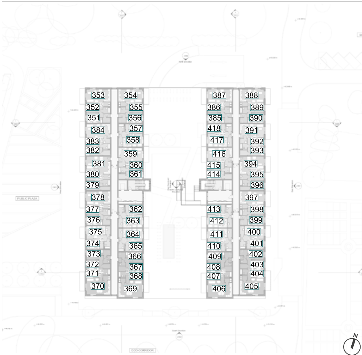
Fig. 19: Floor Plan
