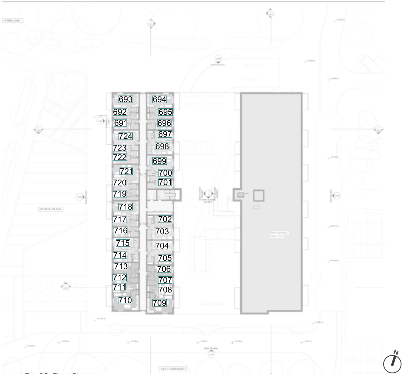
Fig. 28: Floor Plan
