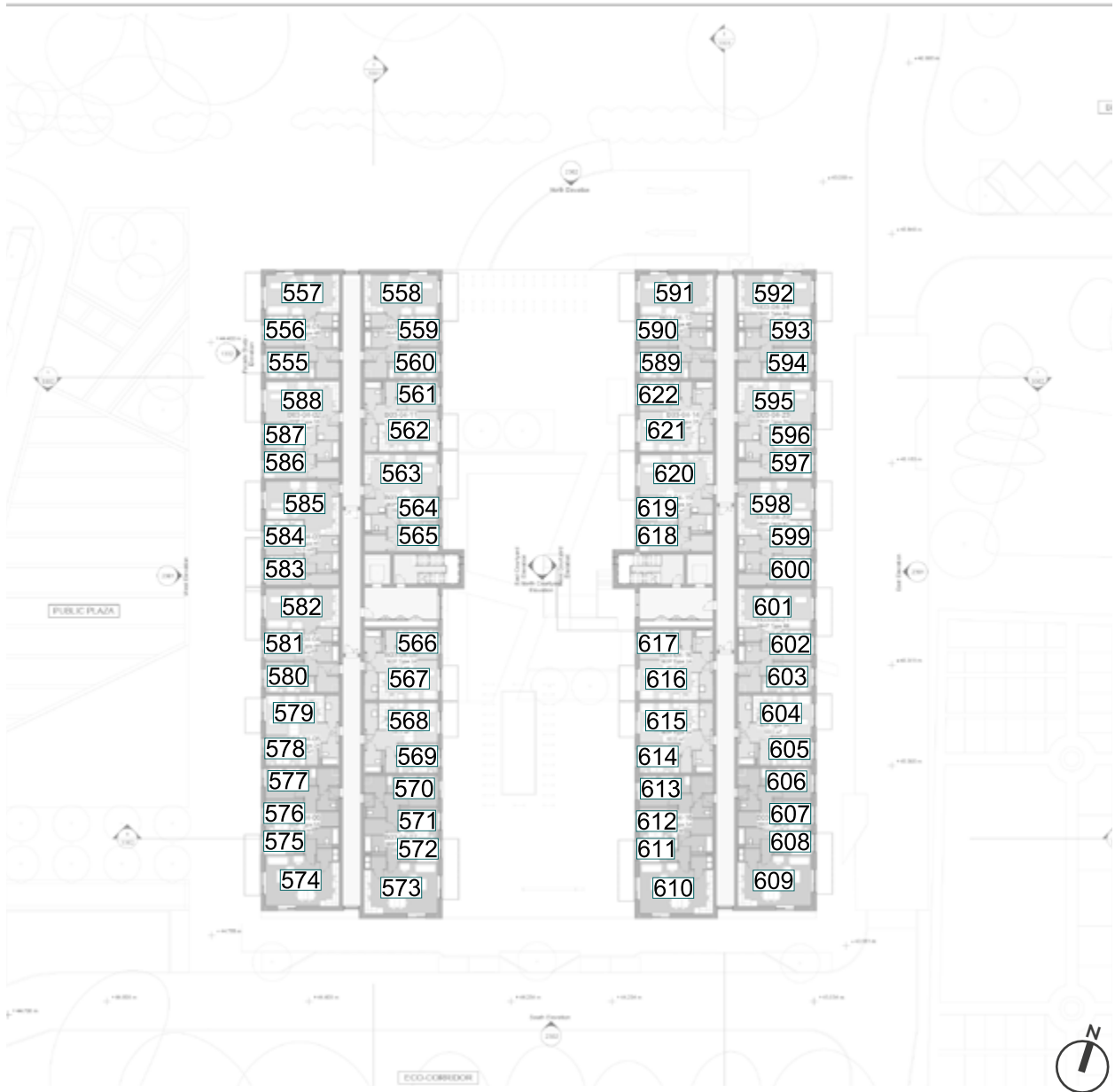
Fig. 25: Floor Plan
