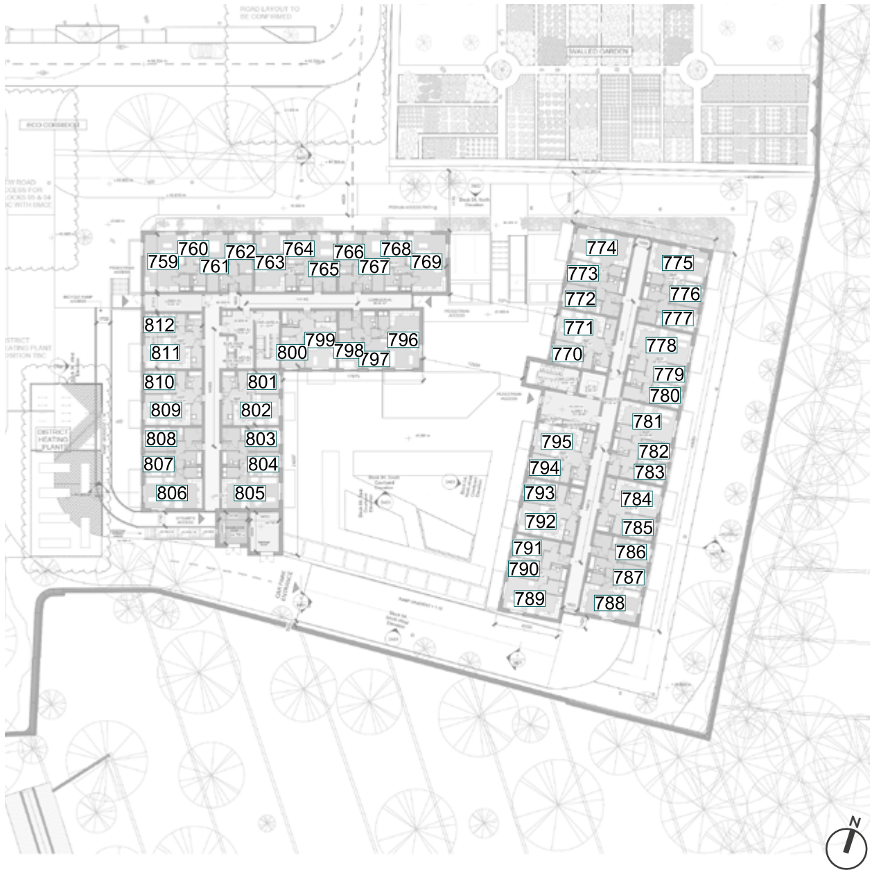
Fig. 31: Floor Plan
