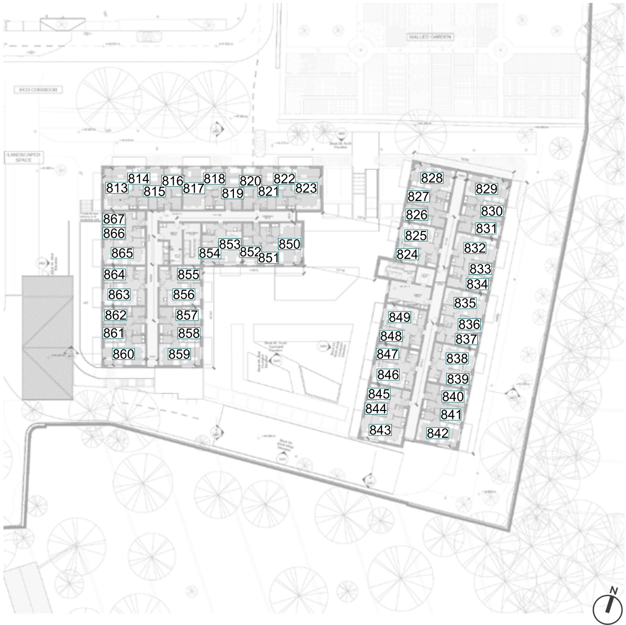
Fig. 32: Floor Plan
