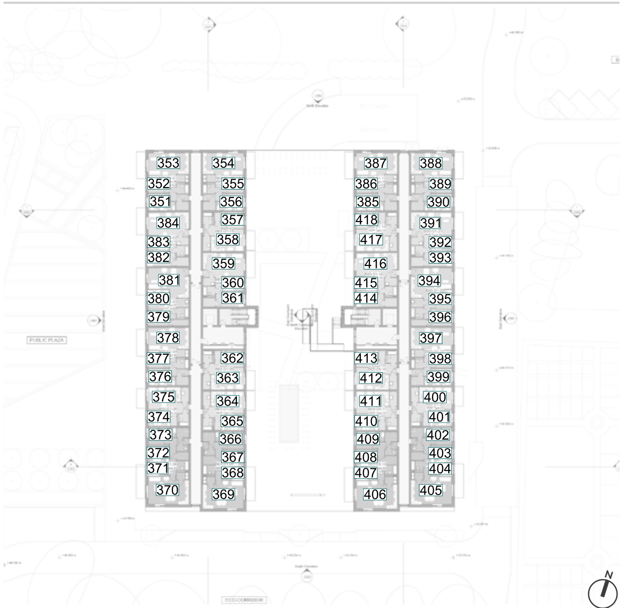
Fig. 18: Floor Plan
