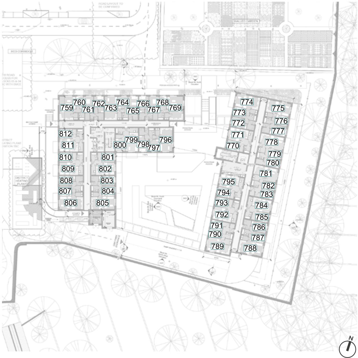
Fig. 30: Floor Plan
